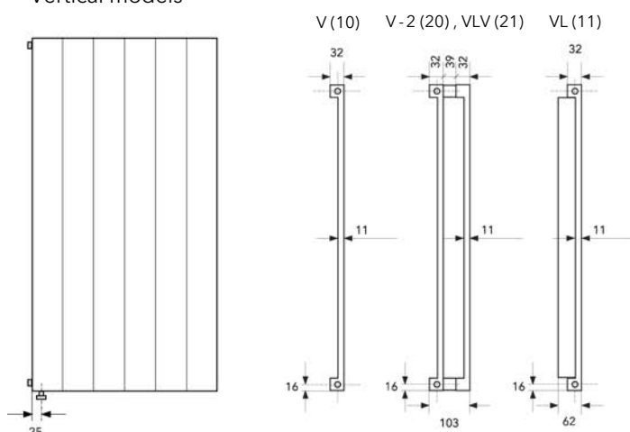
Vertical models
