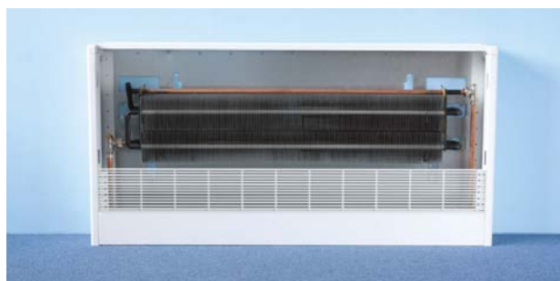
Internal Style C casing with finned element
