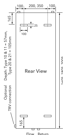
Vertical Types 10, 11, 20 & 21
